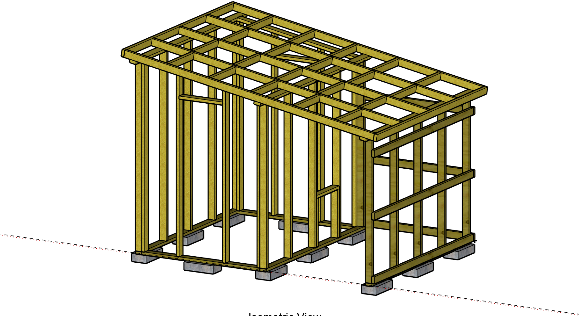
Isometric View
